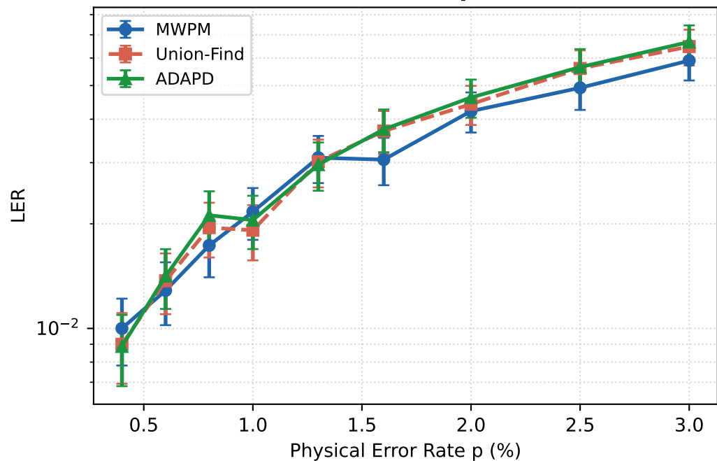
d = 9 (n = 81 qubits)
