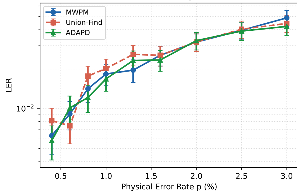
d = 7 (n = 49 qubits)
