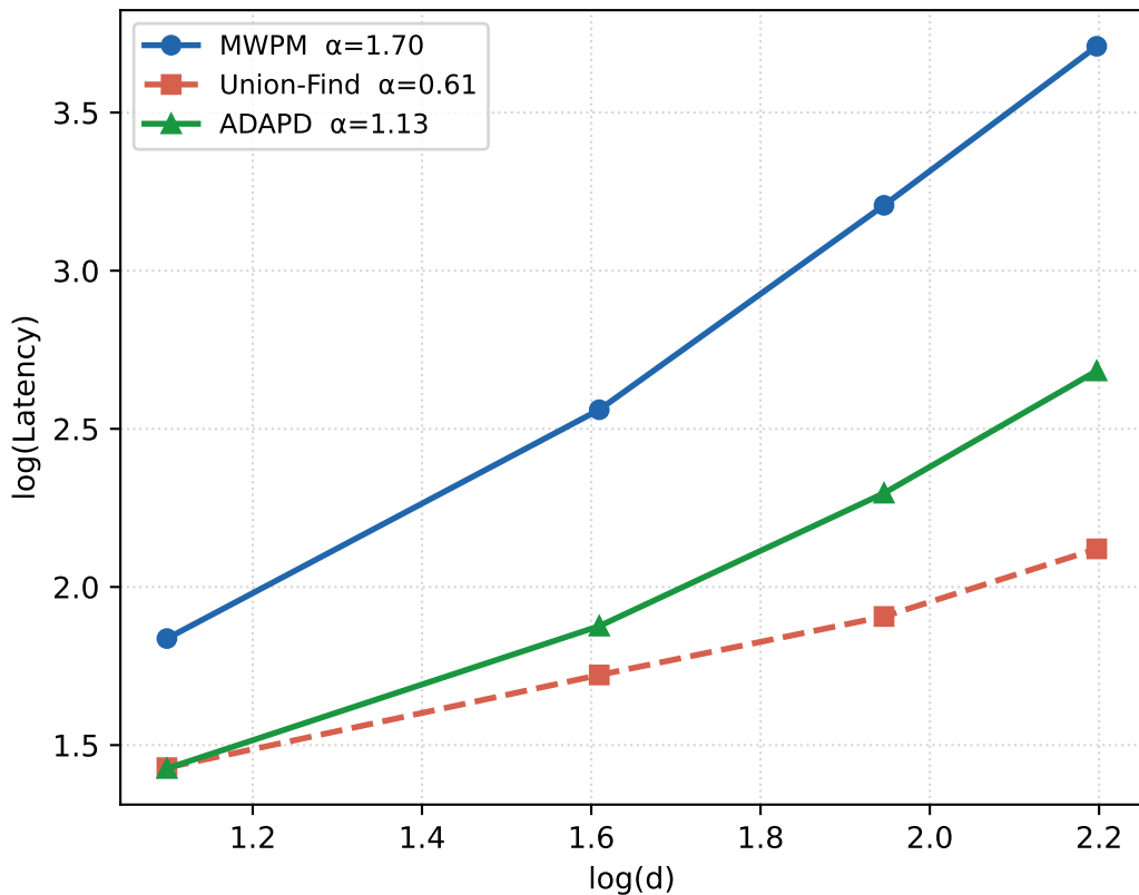
Log-Log Scaling
