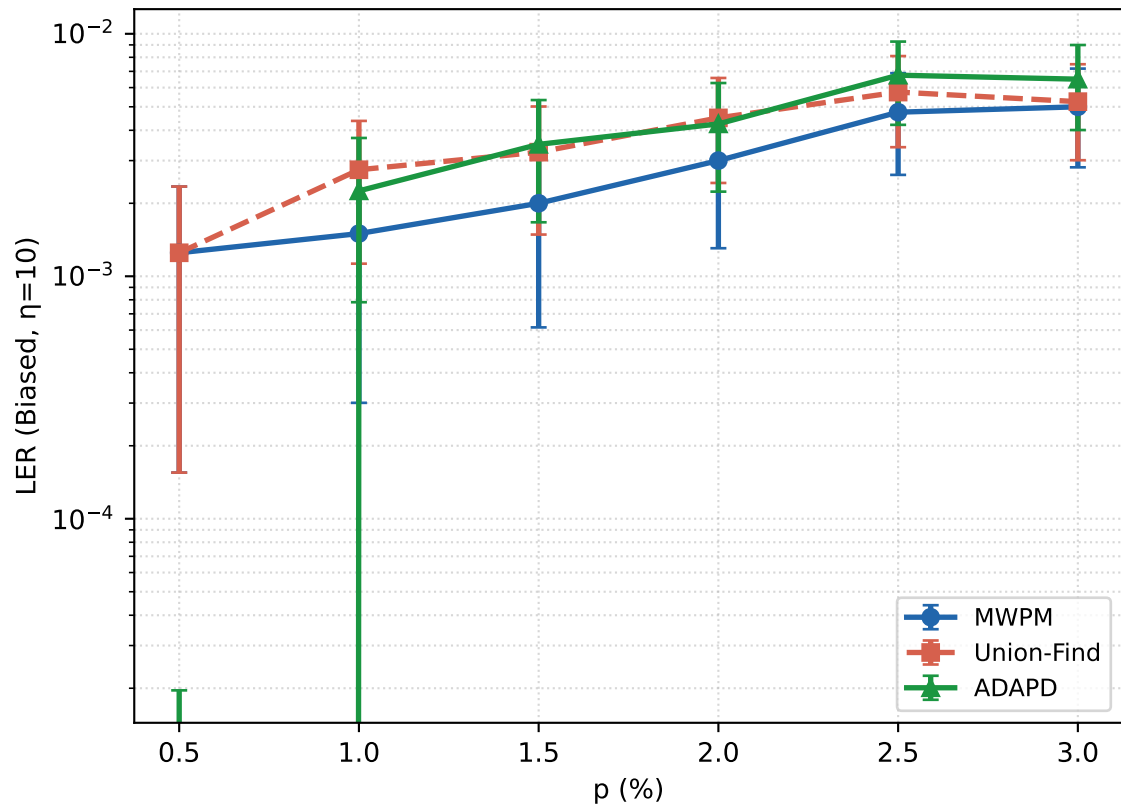
Z-Biased Noise d=7
