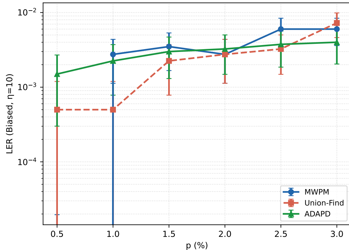
Z-Biased Noise d=5
