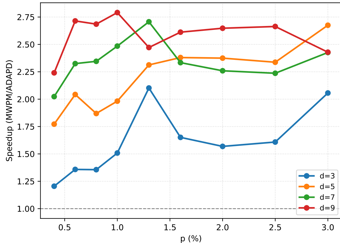
ADAPD Latency Speedup over MWPM
