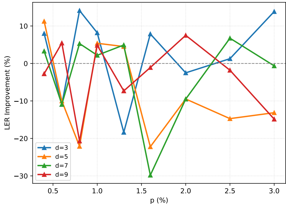
ADAPD LER Improvement over MWPM
