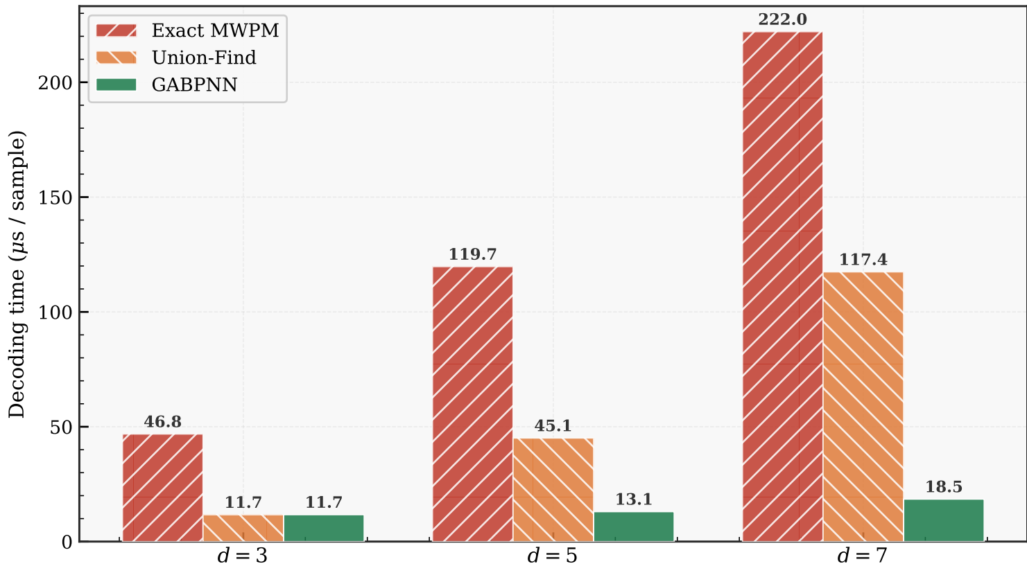
Decoder latency comparison (Python CPU)
