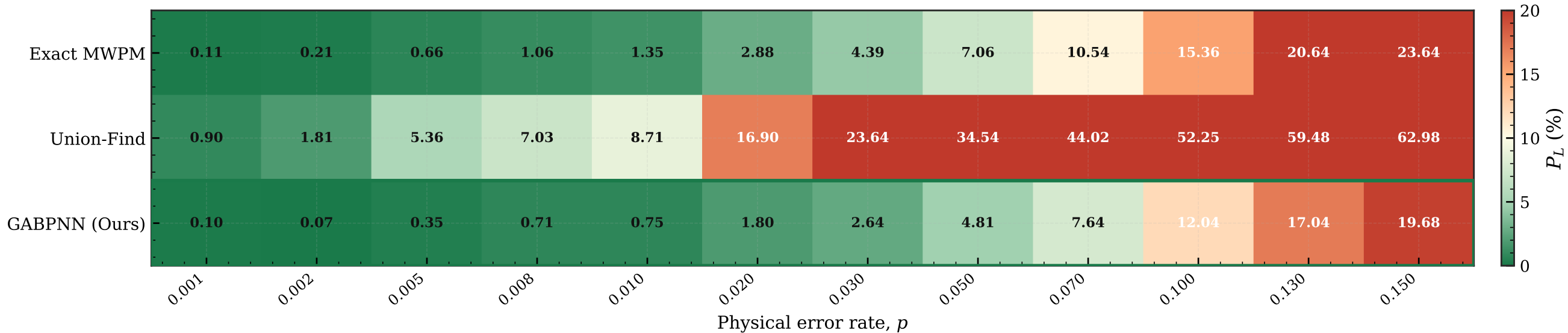
P_L heatmap — d = 5 , symmetric depolarising channel
