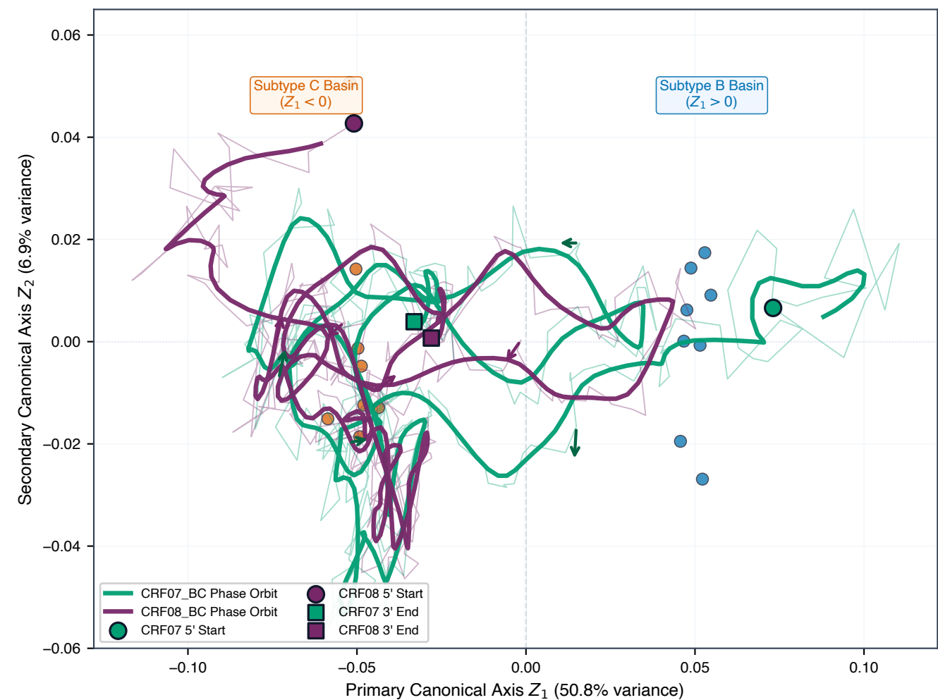
D 2D Metric Phase Space Dynamics ( Z_1 \times Z_2 )
