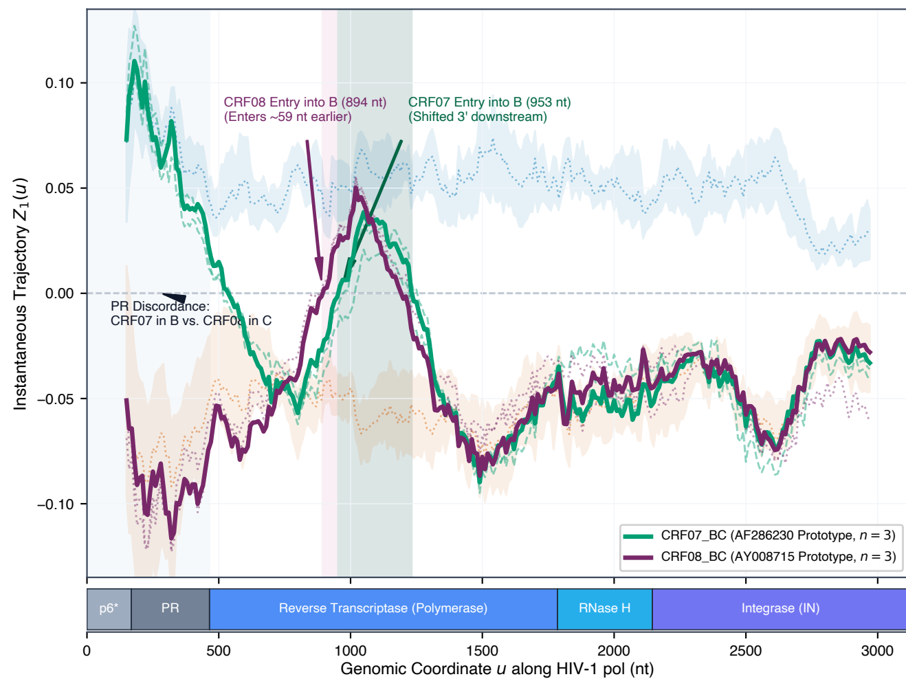
C Dynamic Recombinant Trajectories ( Z_1(u) vs. Parental Corridors)
