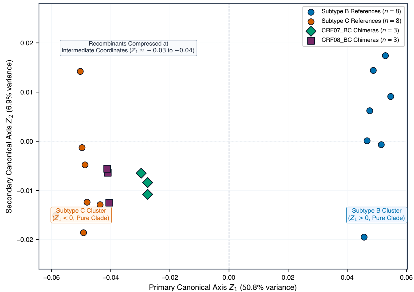
A Global Buneman Metric Space ( N = 22 sequences)
