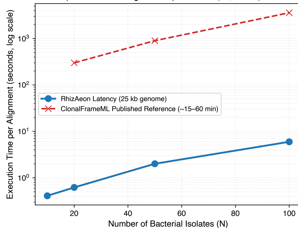
D. Computational Scaling vs Sample Size N (25,000 nt)
