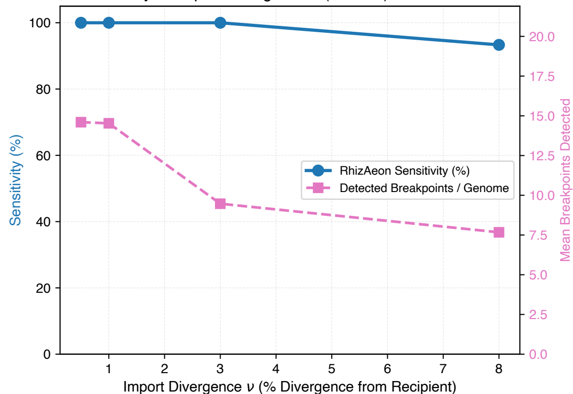
C. Sensitivity vs Import Divergence \nu ( r/m=1.0 )
