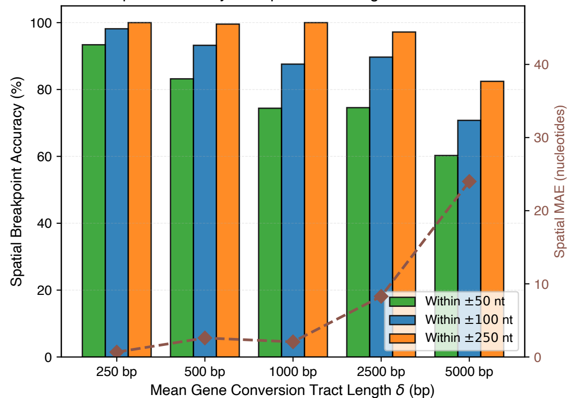
B. Breakpoint Accuracy vs Import Tract Length
