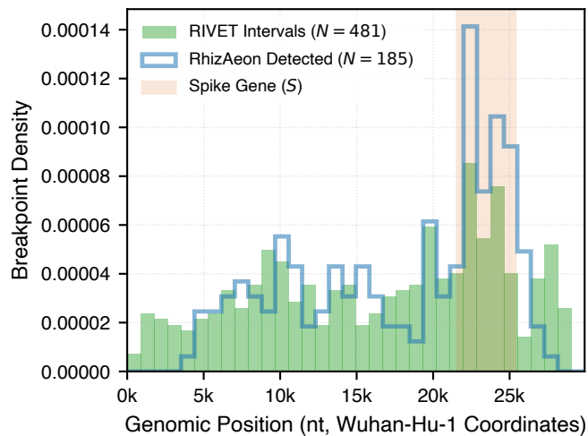
C Empirical Genomic Breakpoint Distribution
