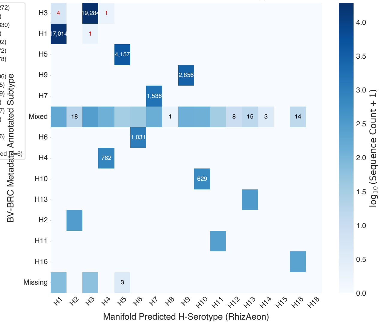
B Serotype Concordance Matrix: Metadata Subtype vs. Manifold Call
