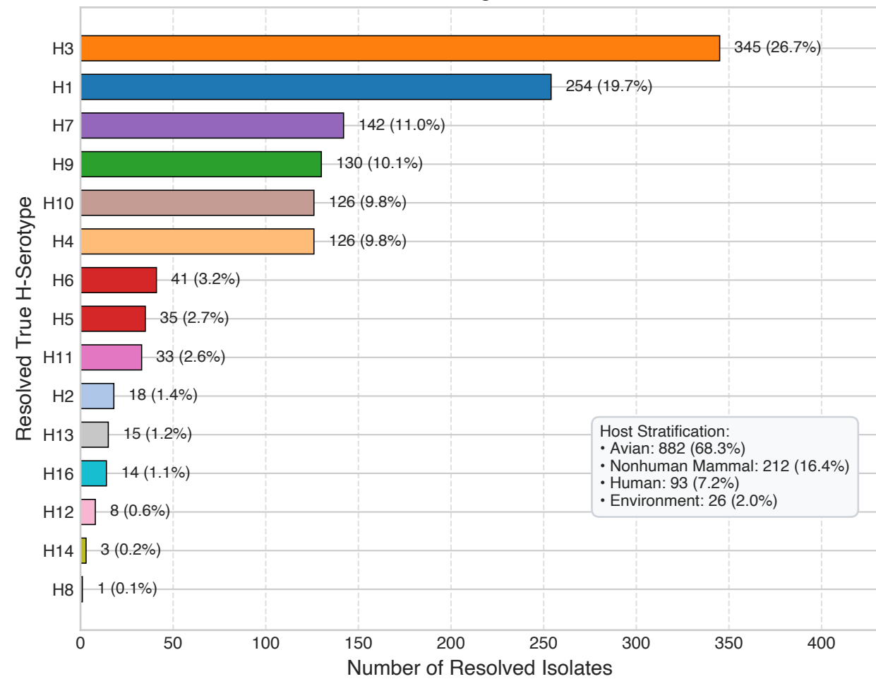
C De Novo Resolution of 1,291 Unassigned &amp; Mixed Field Isolates
