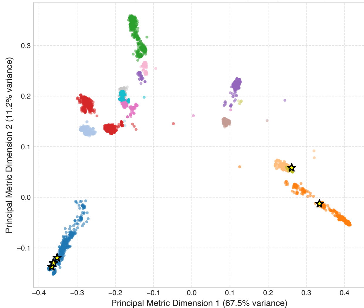
A Whole-Database Sequence Metric Manifold Projection (N = 49,875)
