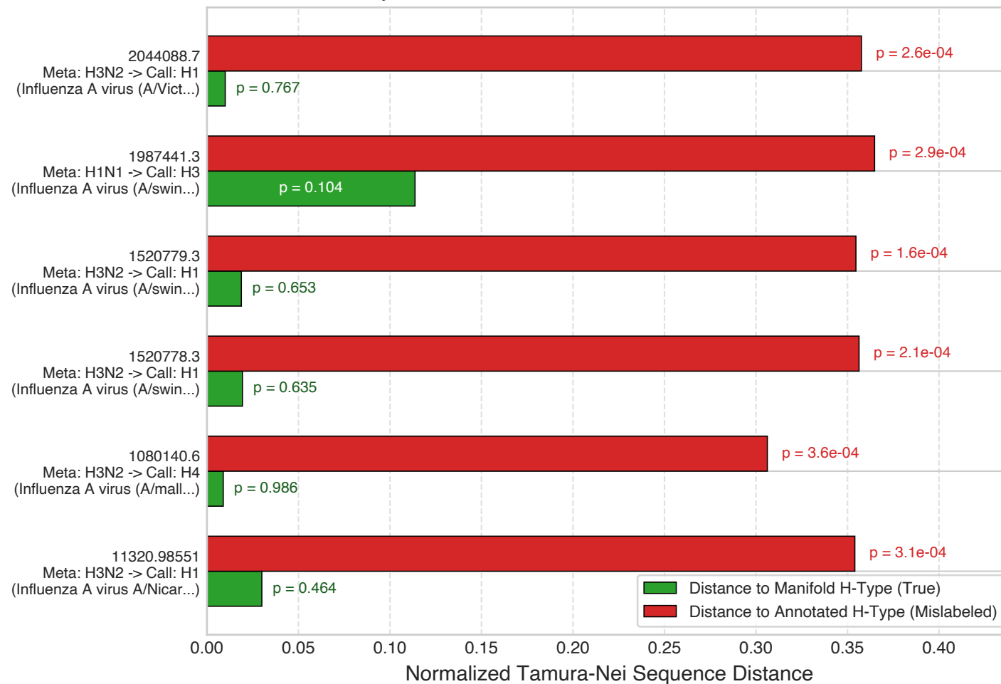
D Conformal Rejection of 6 Metadata Misannotations in BV-BRC
