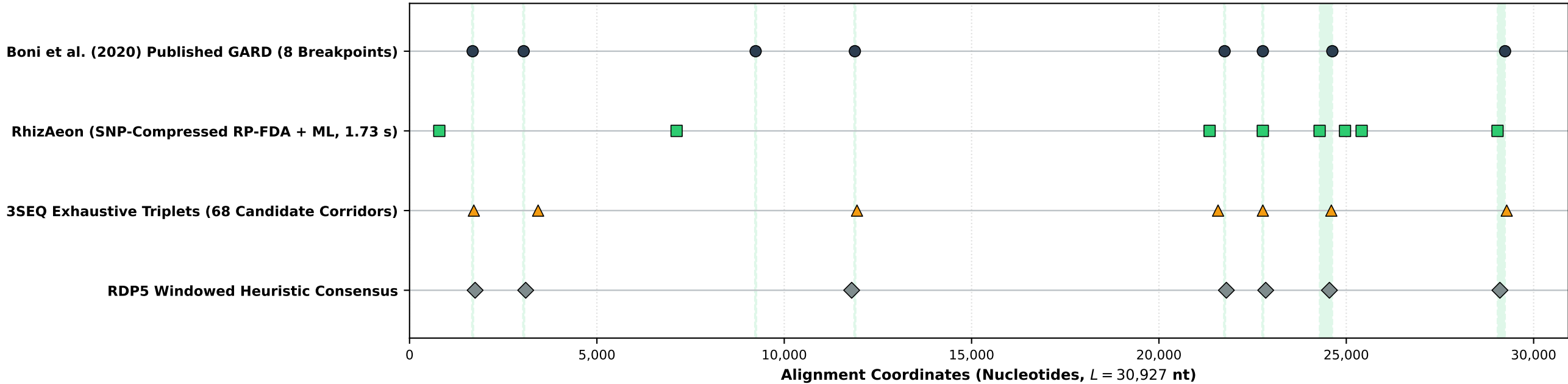
Panel C: Track 3 — Multi-Tool Concordance & Disagreement Horizon (RhizAeon vs GARD vs 3SEQ vs RDP5)
