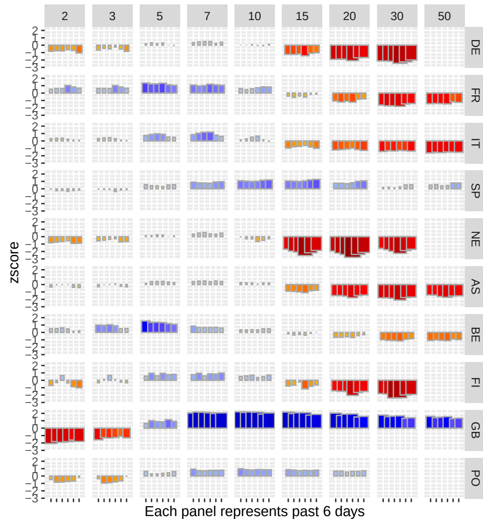
Curve relative value evolution
