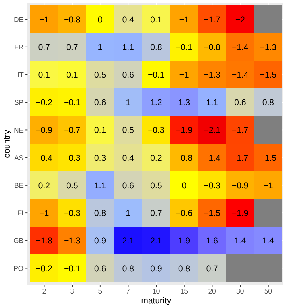
Curve relative value heatmap
