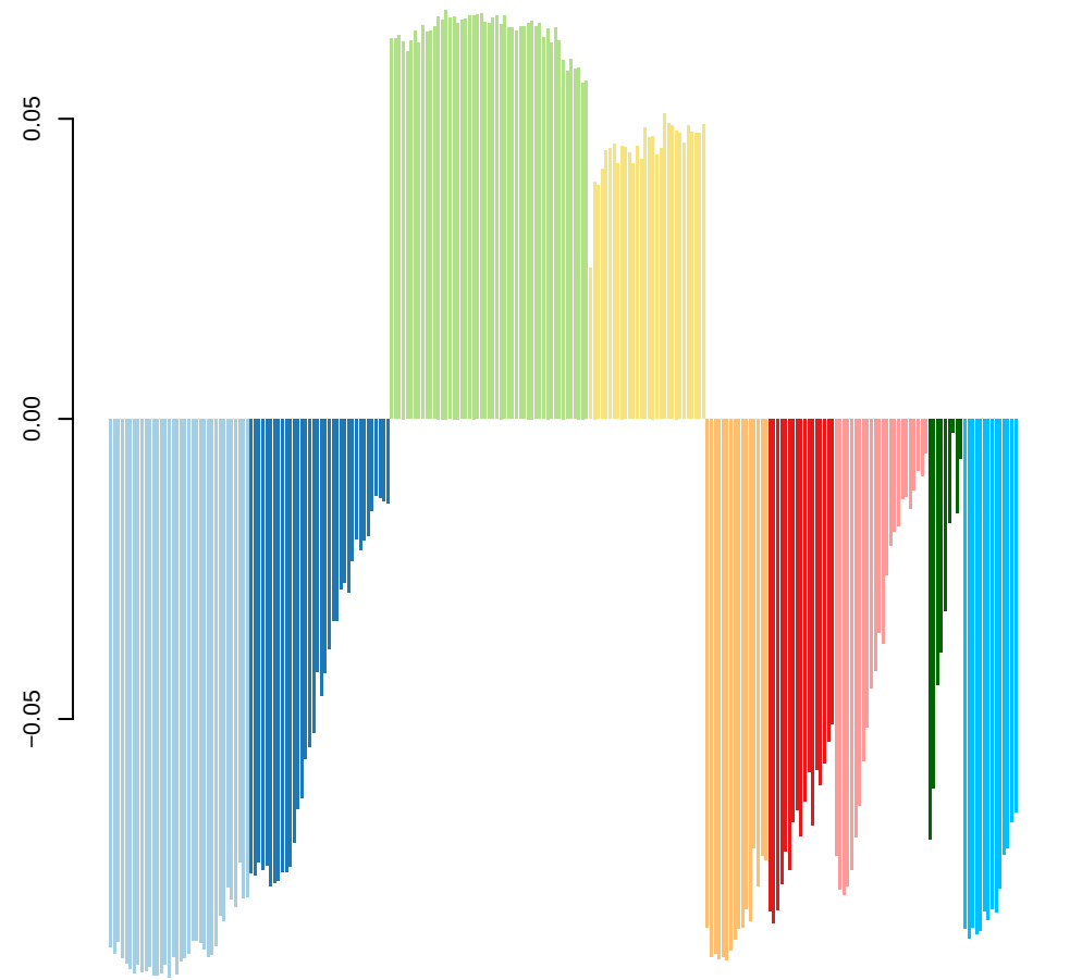
PC1 loadings, variance explained: 45%
