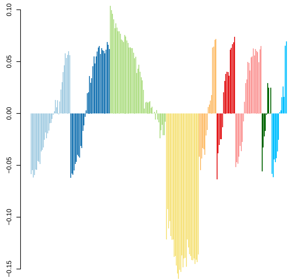
PC4 loadings, variance explained: 5%
