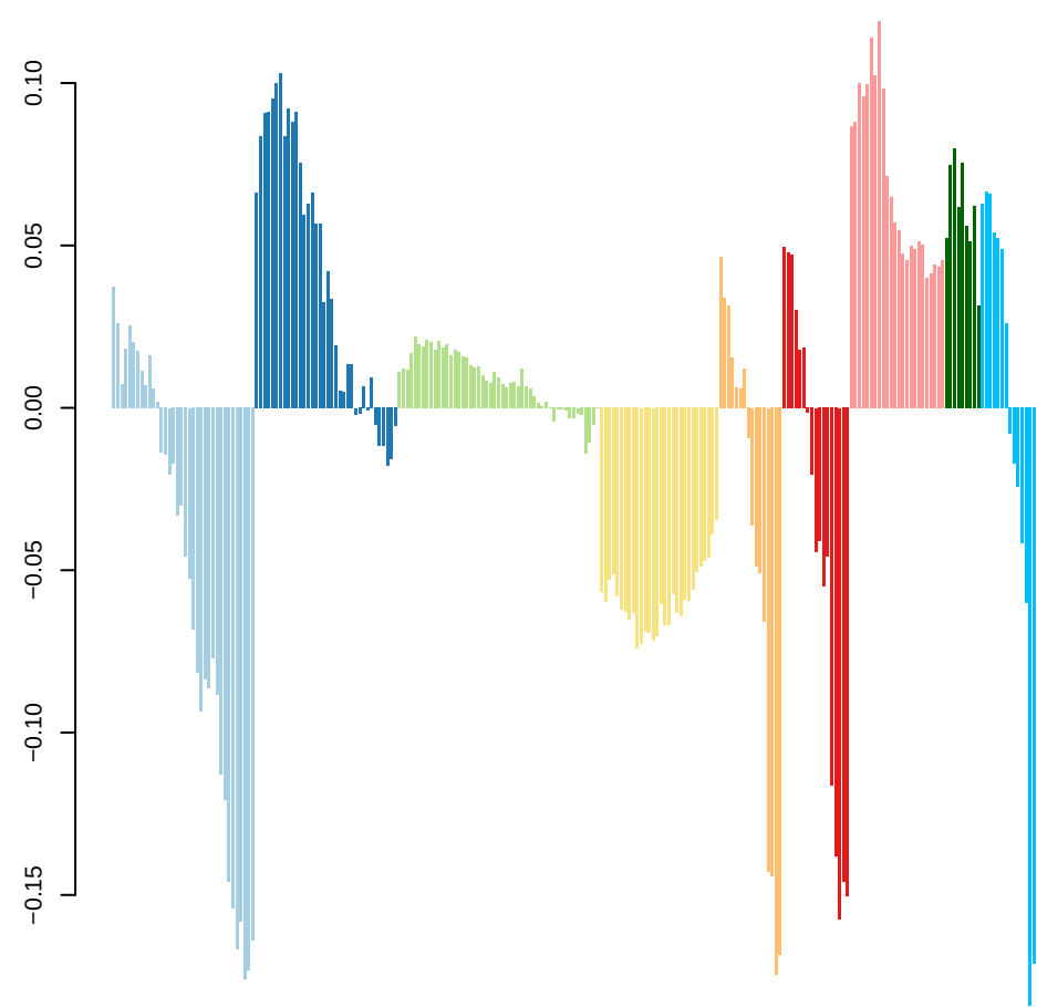
PC5 loadings, variance explained: 3%
