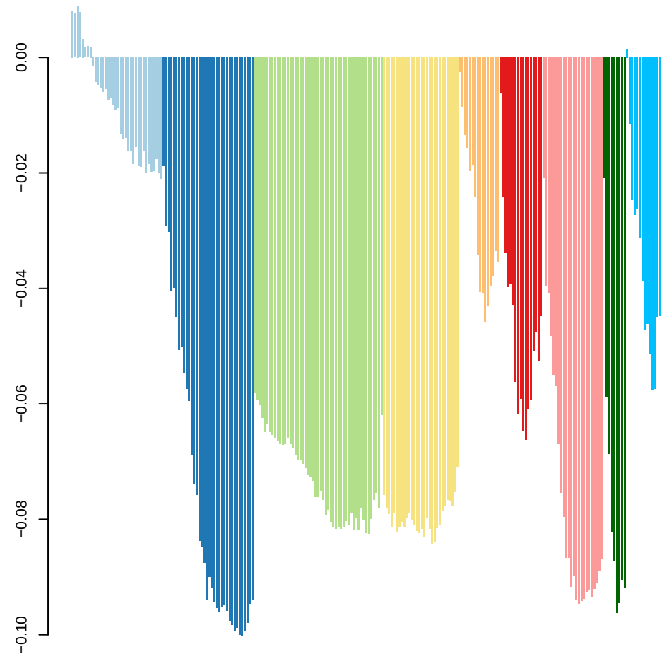
PC2 loadings, variance explained: 29%
