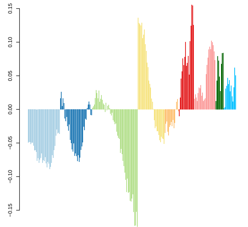
PC6 loadings, variance explained: 2%
