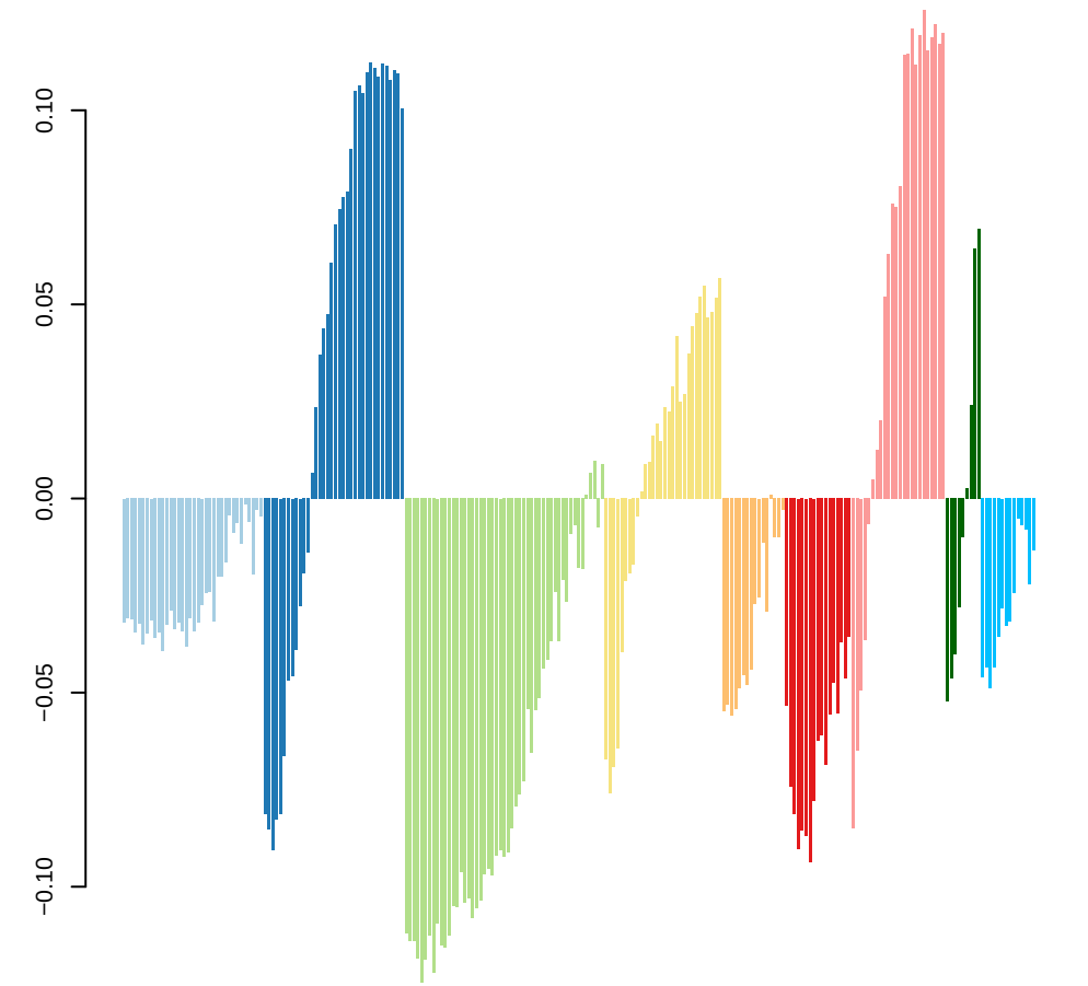
PC3 loadings, variance explained: 6%
