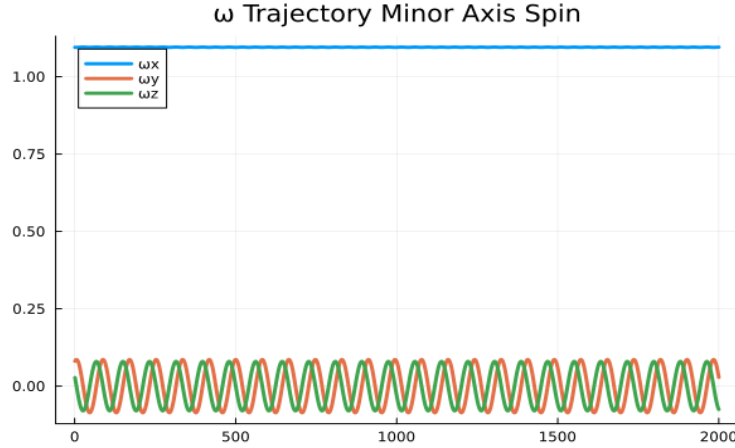
Figure 4: Minor Axis Spin Angular Velocity Trajectory
