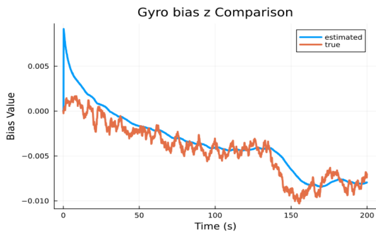
Figure 24: Gyro Bias z component True vs Estimated Plot
