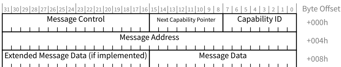
Figure 7-44 MSI Capability Structure for 32-bit Message Address
