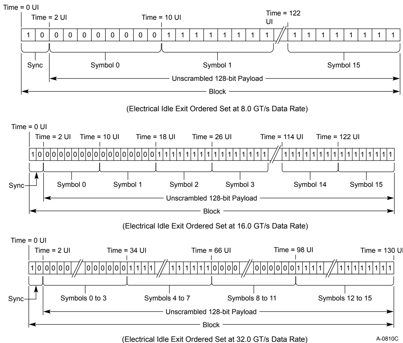
Figure 4-25 Electrical Idle Exit Ordered Set for 8.0 GT/s and Above Data Rates ( EIEOS )
