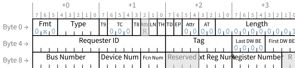
Figure 2-20 Request Header Format for Configuration Transactions
