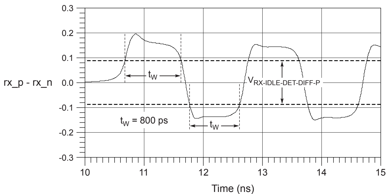
Figure 8-46 Exit from Idle Voltage and Time Margins
