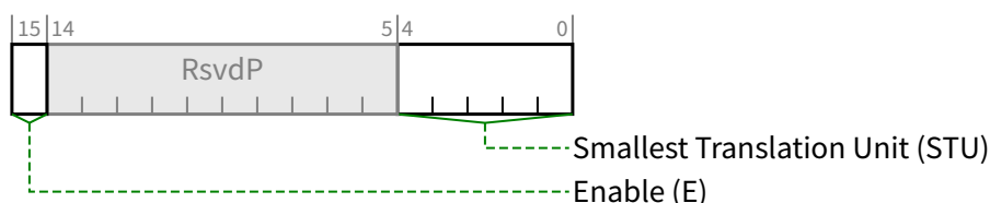
Figure 10-22 ATS Control Register
