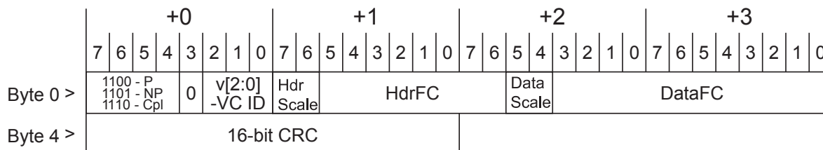
Figure 3-8 Data Link Layer Packet Format for InitFC2
