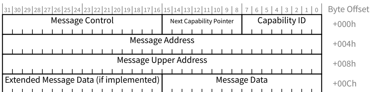
Figure 7-45 MSI Capability Structure for 64-bit Message Address
