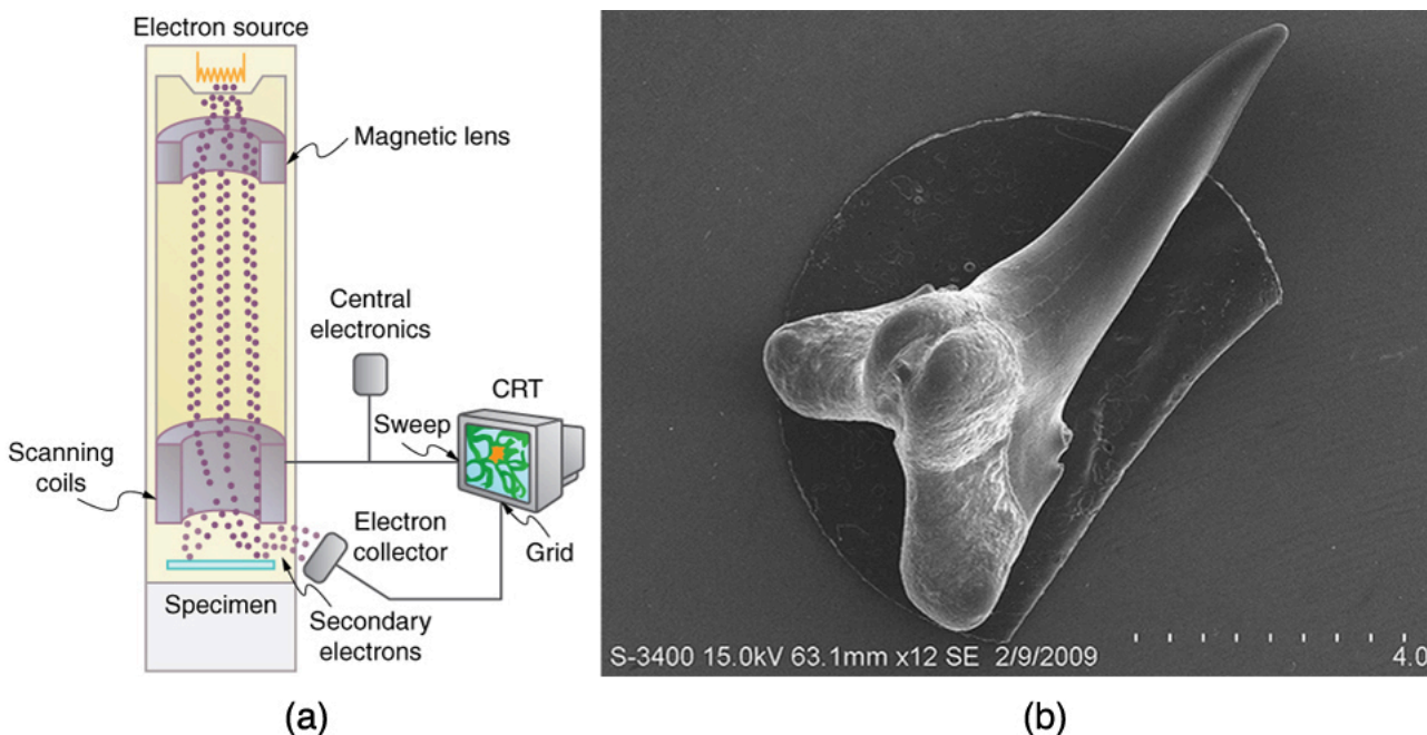
Schematic of a scanning electron microscope (SEM) (a) used to observe small details, such as those seen in this image of a tooth of a Himnirpistis , a type of shark (b). (credit: Dallas Krentzel, Flickr)
