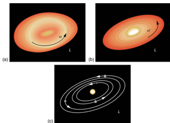
The Solar System coalesced from a cloud of gas and dust that was originally rotating. The orbital motions and spins of the planets are in the same direction as the original spin and conserve the angular momentum of the parent cloud.
