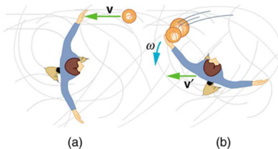
The figure shows the overhead view of a person standing motionless on ice about to catch a ball. Both arms are outstretched. After catching the ball, the skater recoils and rotates.
