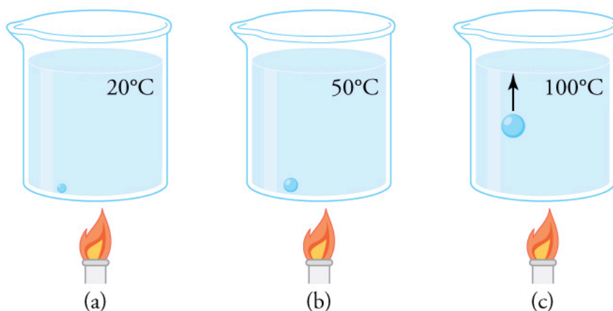
(a) An air bubble in water starts out saturated with water vapor at 20^\circ\text{C} . (b) As the temperature rises, water vapor enters the bubble because its vapor pressure increases. The bubble expands to keep its pressure at 1.00 atm. (c) At 100^\circ\text{C} , water vapor enters the bubble continuously because water's vapor pressure exceeds its partial pressure in the bubble, which must be less than 1.00 atm. The bubble grows and rises to the surface.
