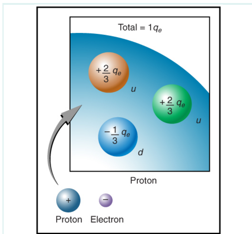
Figure 5: Artist's conception of fractional quark charges inside a proton. A group of three quark charges add up to the single positive charge on the proton: -\frac{1}{3}q_e + \frac{2}{3}q_e + \frac{2}{3}q_e = +1q_e .
