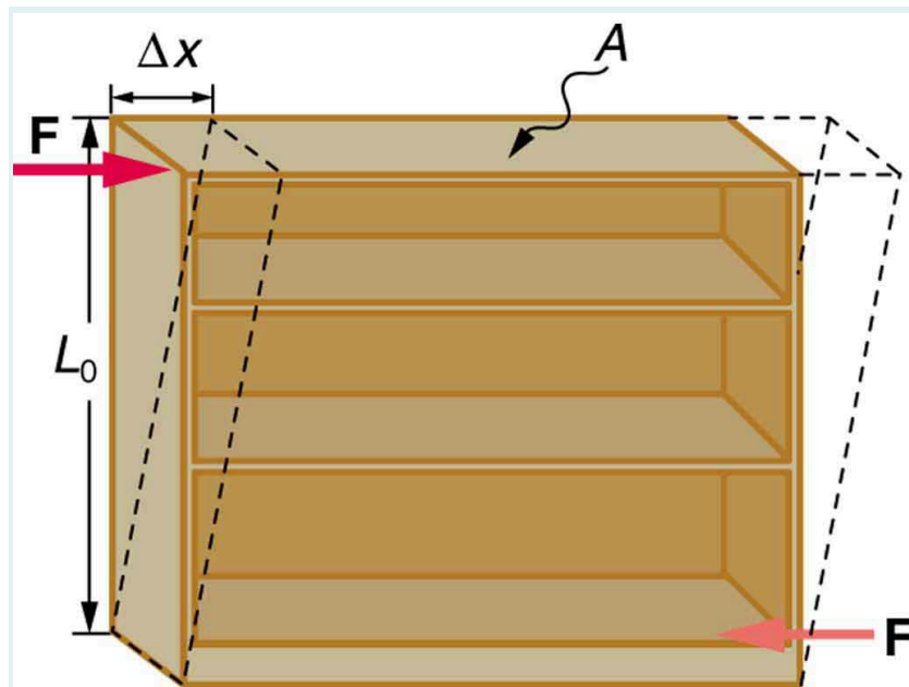
Figure 6: Shearing forces are applied perpendicular to the length (L_0) and parallel to the area (A) , producing a deformation (\Delta x) . Vertical forces are not shown, but it should be kept in mind that in addition to the two shearing forces, (F) , there must be supporting forces to keep the object from rotating. The distorting effects of these supporting forces are ignored in this treatment. The weight of the object also is not shown, since it is usually negligible compared with forces large enough to cause significant deformations.
