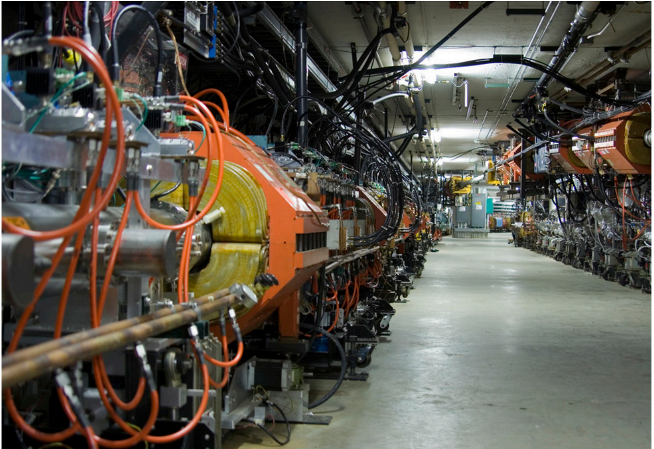
The Fermilab facility in Illinois has a large particle accelerator (the most powerful in the world until 2008) that employs magnetic fields (magnets seen here in orange) to contain and direct its beam. This and other accelerators have been in use for several decades and have allowed us to discover some of the laws underlying all matter. (credit: ammcgrim, Flickr)
