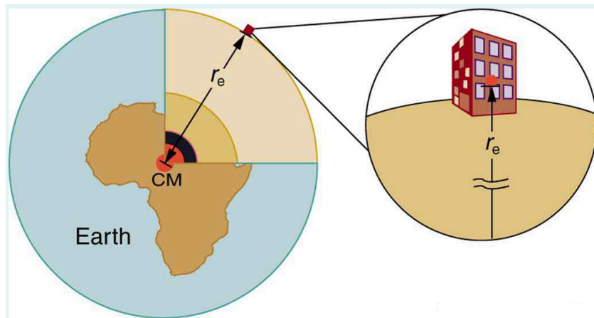
Figure 3: The distance between the centers of mass of Earth and an object on its surface is very nearly the same as the radius of Earth, because Earth is so much larger than the object.
