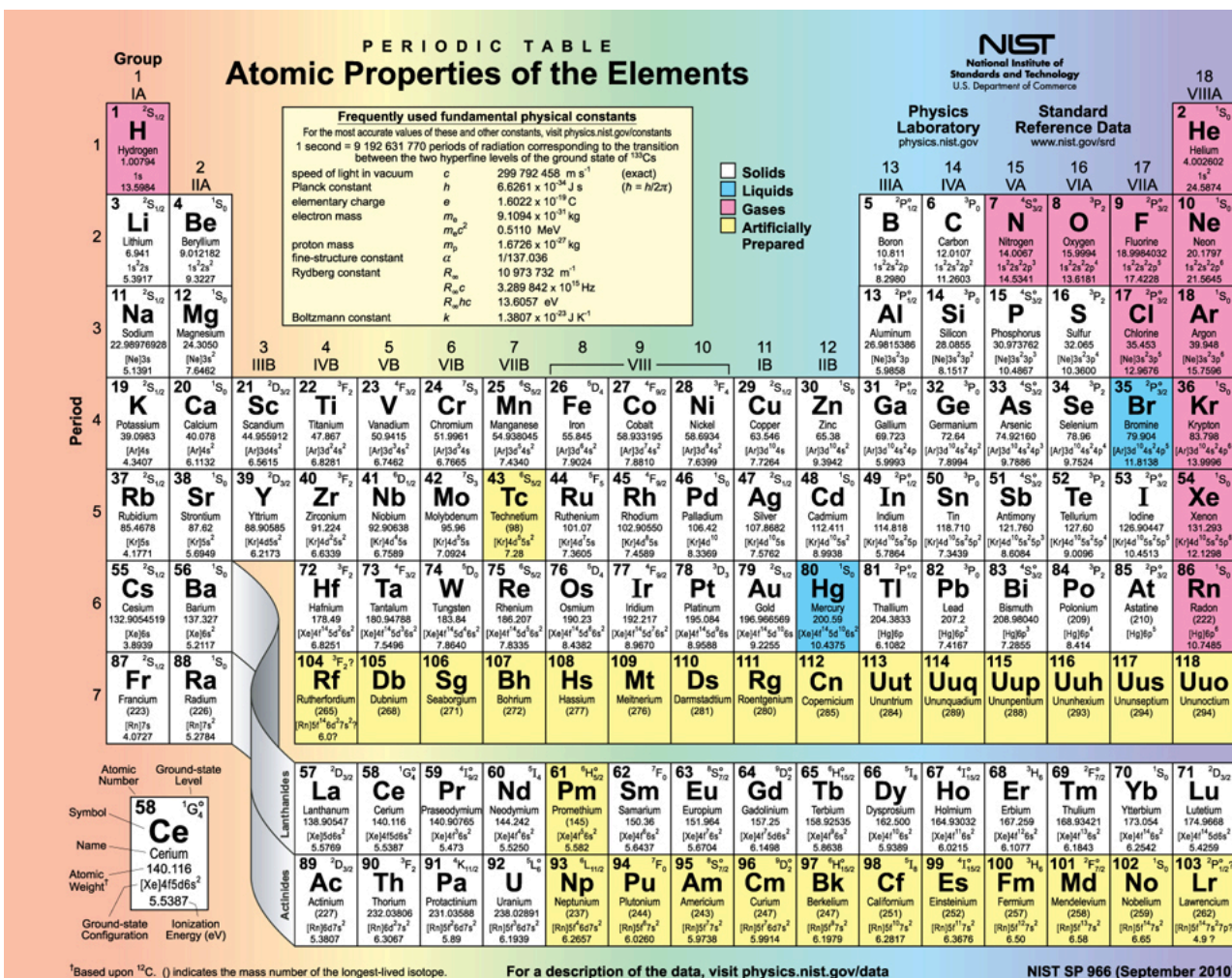
Periodic table of the elements (credit: National Institute of Standards and Technology, U.S. Department of Commerce)
