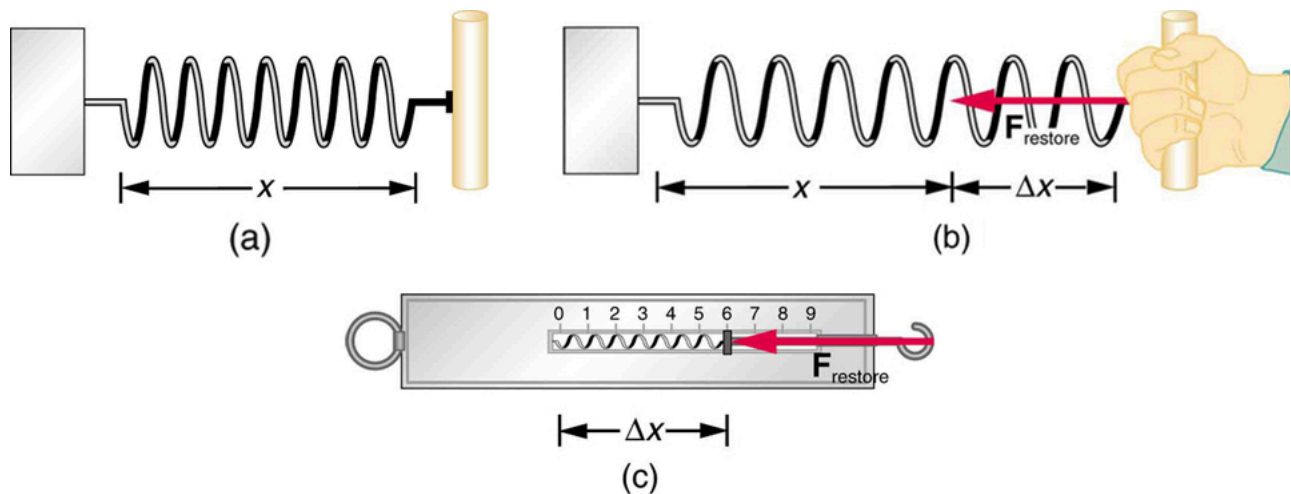
The force exerted by a stretched spring can be used as a standard unit of force. (a) This spring has a length X when undistorted. (b) When stretched a distance \Delta X , the spring exerts a restoring force, F_{\text{restore}} , which is reproducible. (c) A spring scale is one device that uses a spring to measure force. The force F_{\text{restore}} is exerted on whatever is attached to the hook. Here F_{\text{restore}} has a magnitude of 6 units in the force standard being employed.
