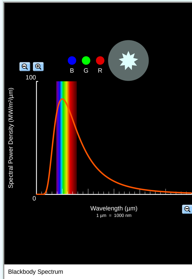
Figure 8: Blackbody Radiation
