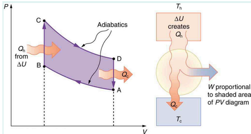
Figure 5: $P$-$V$ diagram for a simplified Otto cycle, analogous to that employed in an internal combustion engine. Point A corresponds to the start of the compression stroke of an internal combustion engine. Paths AB and CD are adiabatic and correspond to the compression and power strokes of an internal combustion engine, respectively. Paths BC and DA are isochoric and accomplish
