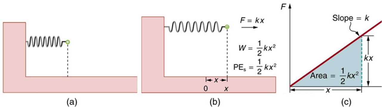
(a) An undeformed spring has no PE_S stored in it. (b) The force needed to stretch (or compress) the spring a distance x has a magnitude F = kx , and the work done to stretch (or compress) it is \frac{1}{2}kx^2 . Because the force is conservative, this work is stored as potential energy, PE_S , in the spring, and it can be fully recovered. (c) A graph of F vs. x has a slope of k , and the area under the graph is \frac{1}{2}kx^2 . Thus the work done or potential energy stored is \frac{1}{2}kx^2 .
