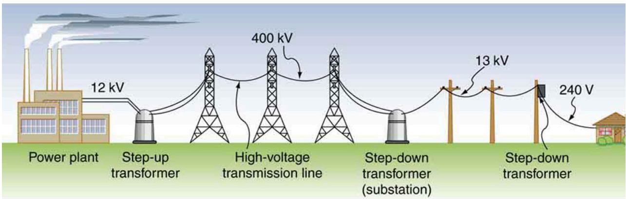
Transformers change voltages at several points in a power distribution system. Electric power is usually generated at greater than 10 kV, and transmitted long distances at voltages over 200 kV—sometimes as great as 700 kV—to limit energy losses. Local power distribution to neighborhoods or industries goes through a substation and is sent short distances at voltages ranging from 5 to 13 kV. This is reduced to 120, 240, or 480 V for safety at the individual user site.
