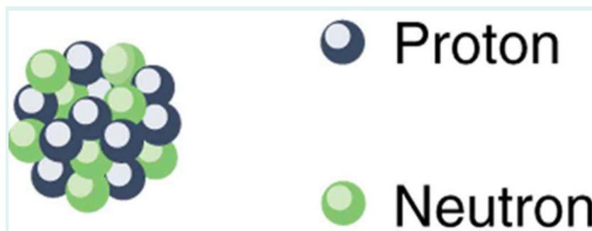
Figure 2: A model of the nucleus.
