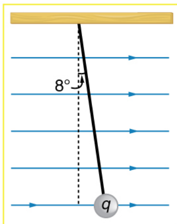
A horizontal electric field causes the charged ball to hang at an angle of 8.00^\circ .
