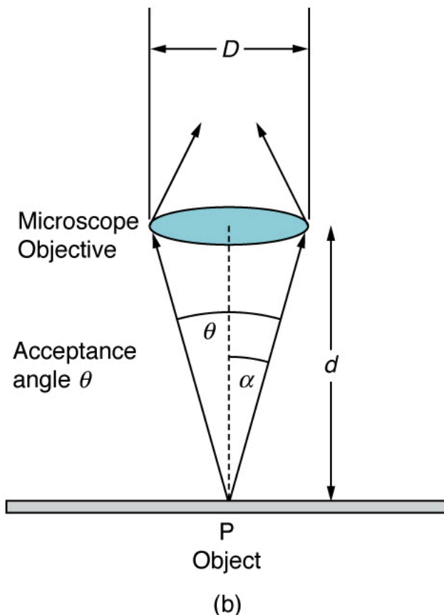
(a) Two points separated by at distance x and a positioned a distance d away from the objective. (credit: Infopro, Wikimedia Commons) (b) Terms and symbols used in discussion of resolving power for a lens and an object at point P. (credit: Infopro, Wikimedia Commons)
