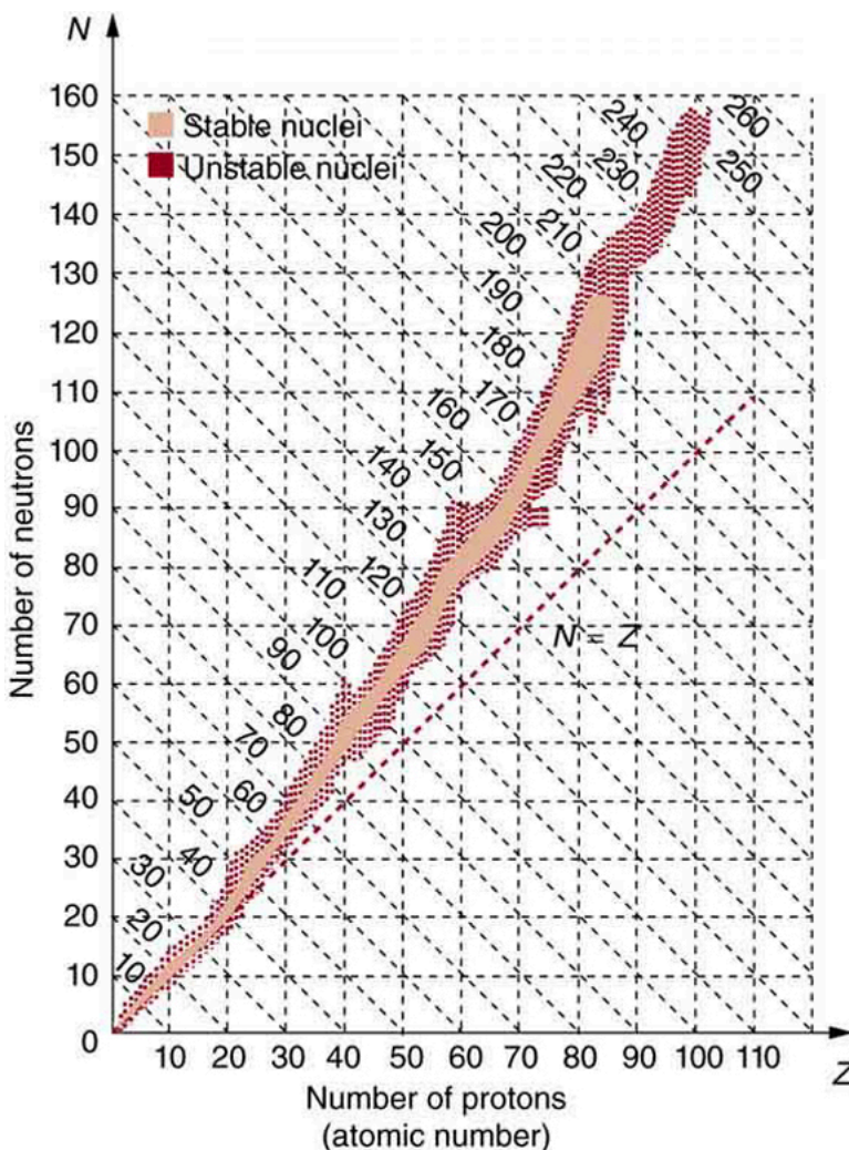
Simplified chart of the nuclides, a graph of N versus Z for known nuclides. The patterns of stable and unstable nuclides reveal characteristics of the nuclear forces. The dashed line is for N = Z . Numbers along diagonals are mass numbers A .
