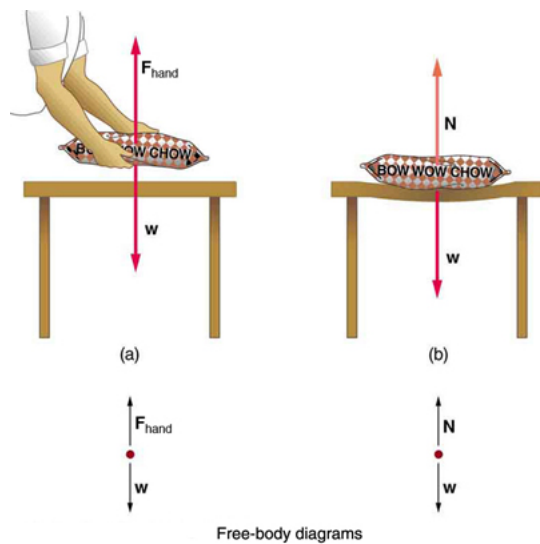
(a) The person holding the bag of dog food must supply an upward force \vec{F}_{\text{hand}} equal in magnitude and opposite in direction to the weight of the food \vec{w} . (b) The card table sags when the dog food is placed on it, much like a stiff trampoline. Elastic restoring forces in the table grow as it sags until they supply a force \vec{N} equal in magnitude and opposite in direction to the weight of the load.
