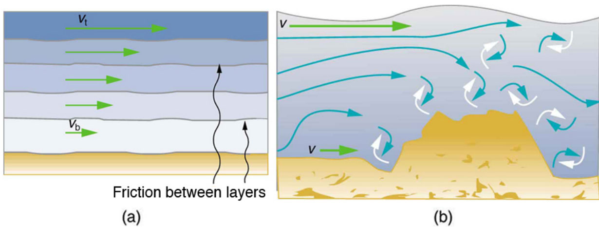
(a) Laminar flow occurs in layers without mixing. Notice that viscosity causes drag between layers as well as with the fixed surface. (b) An obstruction in the vessel produces turbulence. Turbulent flow mixes the fluid. There is more interaction, greater heating, and more resistance than in laminar flow.
