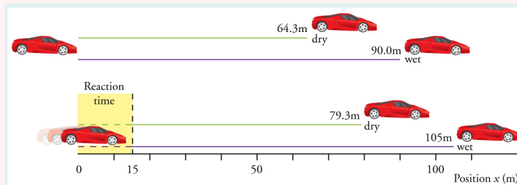
Figure 6: The distance necessary to stop a car varies greatly, depending on road conditions and driver reaction time. Shown here are the braking distances for dry and wet pavement, as calculated in this example, for a car initially traveling at 30.0 m/s. Also shown are the total distances traveled from the point where the driver first sees a light turn red, assuming a 0.500 s reaction time.
