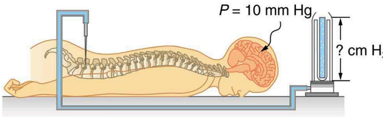
A water manometer used to measure pressure in the spinal fluid. The height of the fluid in the manometer is measured relative to the spinal column, and the manometer is open to the atmosphere. The measured pressure will be considerably greater if the person sits up.
