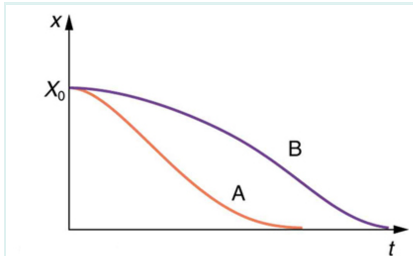
Figure 3: Displacement versus time for a critically damped harmonic oscillator (A) and an overdamped harmonic oscillator (B). The critically damped oscillator returns to equilibrium at x=0 in the smallest time possible without overshooting.
