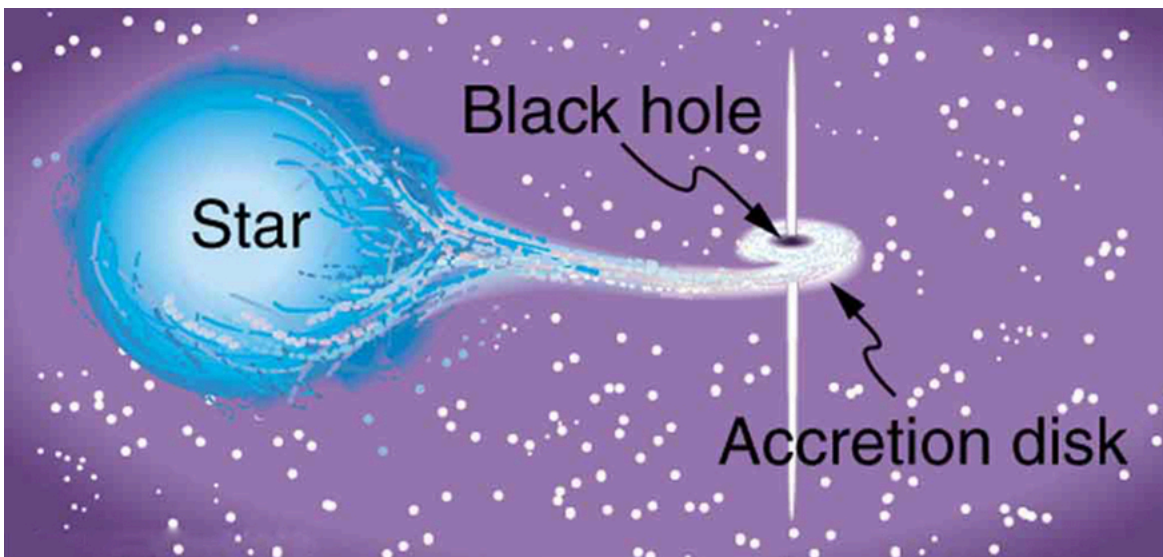
A black hole is shown pulling matter away from a companion star, forming a superheated accretion disk where X-rays are emitted before the matter disappears forever into the hole. The in-fall energy also ejects some material, forming the two vertical spikes. (See also the photograph in Introduction to Frontiers of Physics.) There are several X-ray-emitting objects in space that are consistent with this picture and are likely to be black holes.
