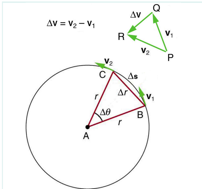
Figure 1: The directions of the velocity of an object at two different points are shown, and the change in velocity \Delta v is seen to point directly toward the center of curvature. (See small inset.) Because a_c = \frac{\Delta v}{\Delta t} , the acceleration is also toward the center; a_c is called centripetal acceleration. (Because \Delta \theta is very small, the arc length \Delta s is equal to the chord length \Delta r for small time differences.)
