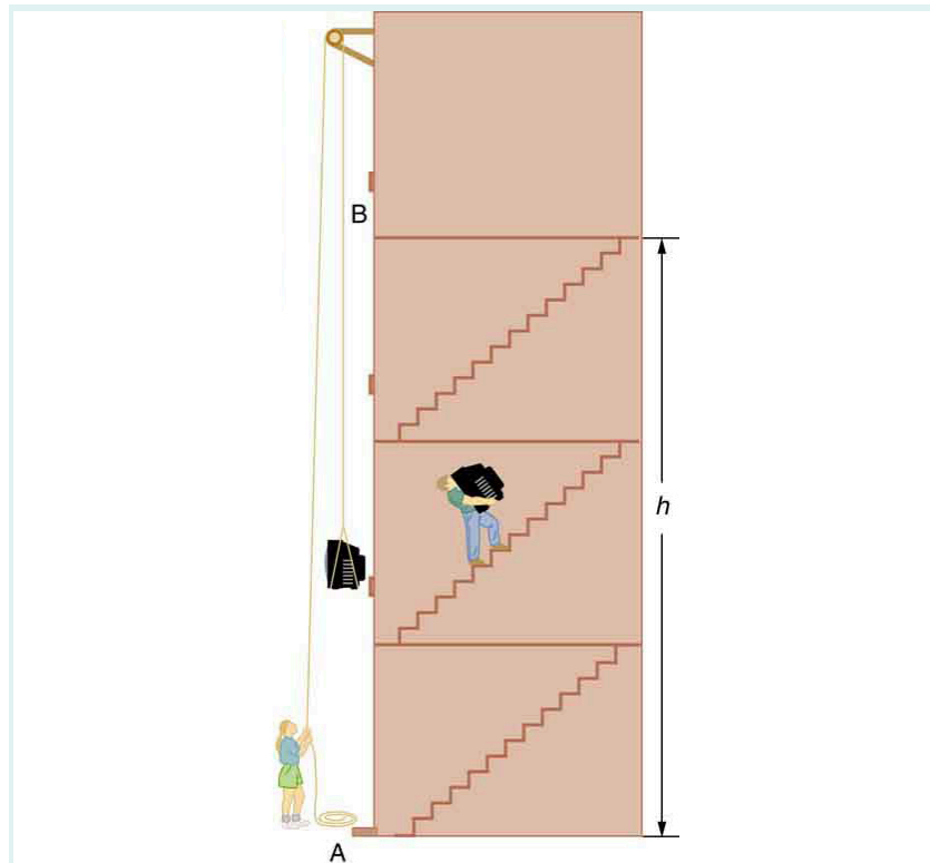
Figure 2: The change in gravitational potential energy \Delta PE_{\text{grav}} between points A and B is independent of the path. \Delta PE_{\text{grav}} = mgh for any path between the two points. Gravity is one of a small class of forces where the work done by or against the force depends only on the starting and ending points, not on the path between them.
