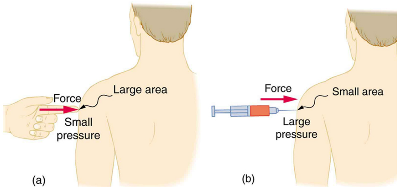
(a) While the person being poked with the finger might be irritated, the force has little lasting effect. (b) In contrast, the same force applied to an area the size of the sharp end of a needle is great enough to break the skin.
