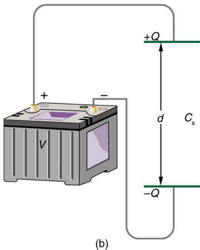
(a) Capacitors connected in series. The magnitude of the charge on each plate is Q . (b) An equivalent capacitor has a larger plate separation d . Series connections produce a total capacitance that is less than that of any of the individual capacitors.
