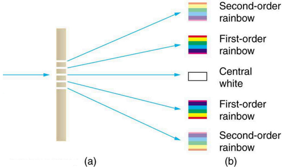
A diffraction grating is a large number of evenly spaced parallel slits. (a) Light passing through is diffracted in a pattern similar to a double slit, with bright regions at various angles. (b) The pattern obtained for white light incident on a grating. The central maximum is white, and the higher-order maxima disperse white light into a rainbow of colors.
