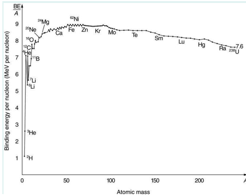
Figure 3: A graph of average binding energy per nucleon, \text{BE}/A , for stable nuclei. The most tightly bound nuclei are those with A near 60, where the attractive nuclear force has its greatest effect. At higher A 's, the Coulomb repulsion progressively reduces the binding energy per nucleon, because the nuclear force is short ranged. The spikes on the curve are very tightly bound nuclides and indicate shell closures.
