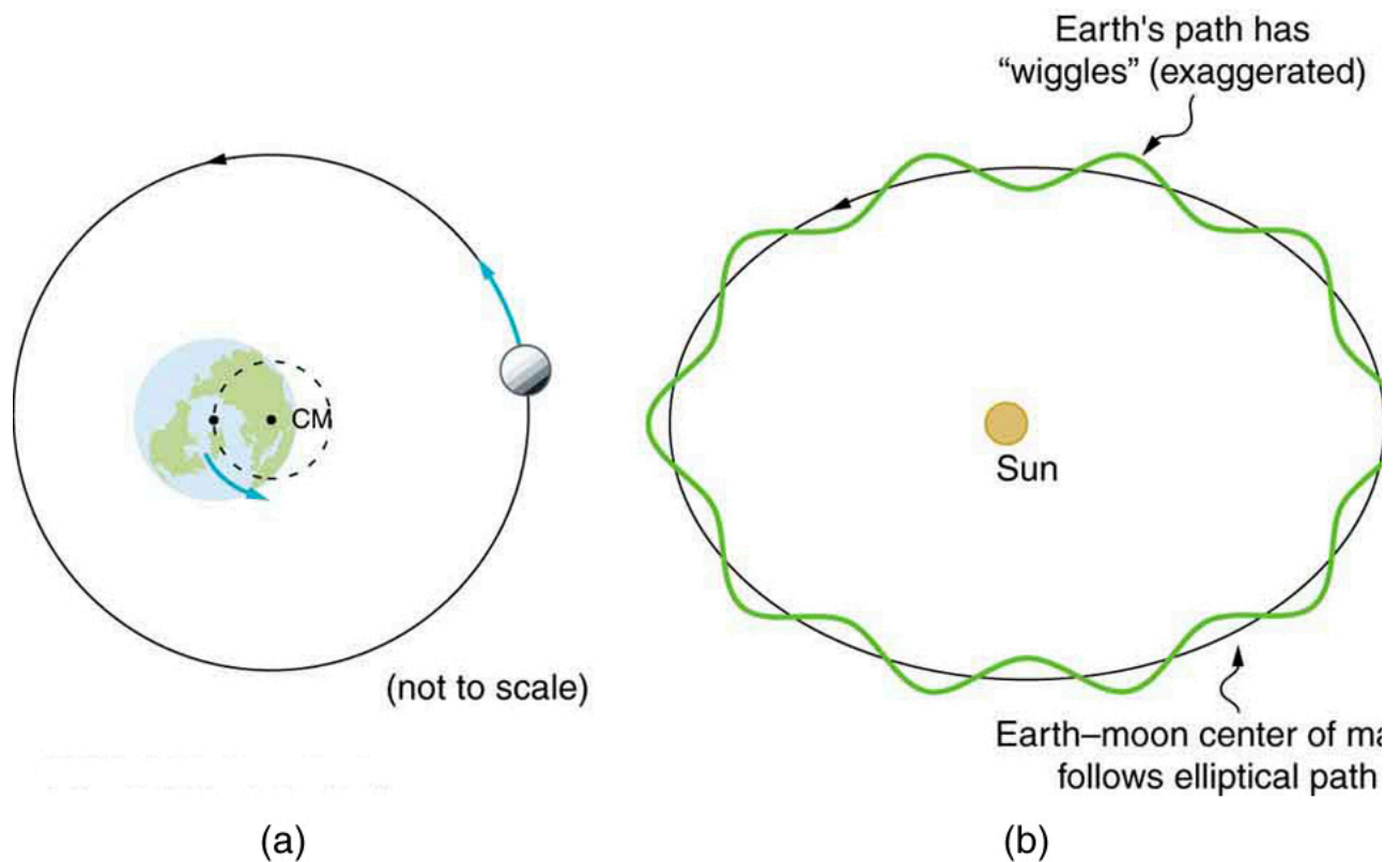
(a) Earth and the Moon rotate approximately once a month around their common center of mass. (b) Their center of mass orbits the Sun in an elliptical orbit, but Earth's path around the Sun has "wiggles" in it. Similar wiggles in the paths of stars have been observed and are considered direct evidence of planets orbiting those stars. This is important because the planets' reflected light is often too dim to be observed.
