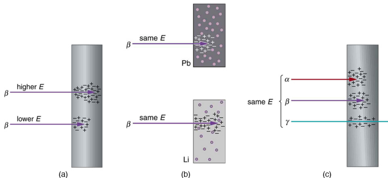
The penetration or range of radiation depends on its energy, the material it encounters, and the type of radiation. (a) Greater energy means greater range. (b) Radiation has a smaller range in materials with high electron density. (c) Alphas have the smallest range, betas have a greater range, and gammas penetrate the farthest.
