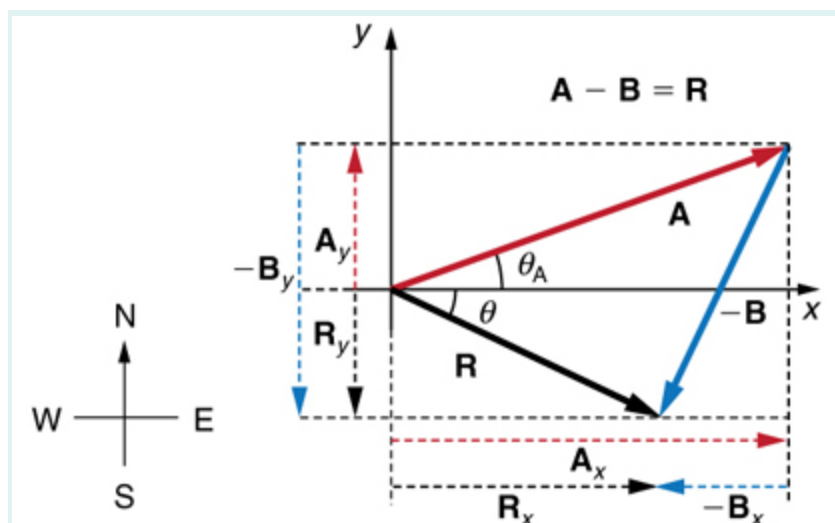
Figure 10: The subtraction of the two vectors shown in Figure 8 . The components of -\vec{B} are the negatives of the components of \vec{B} . The method of subtraction is the same as that for addition.
