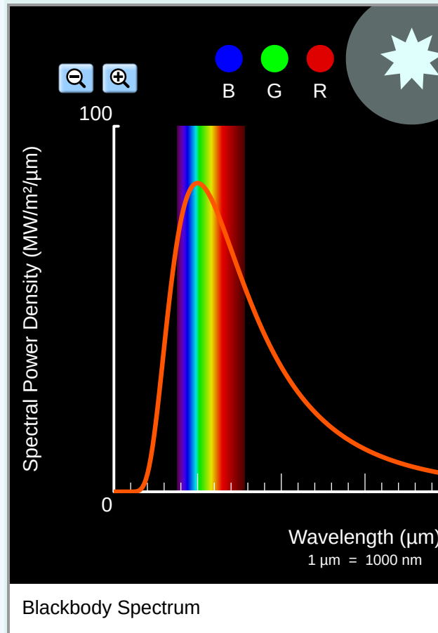
Figure 8: Blackbody Radiation
