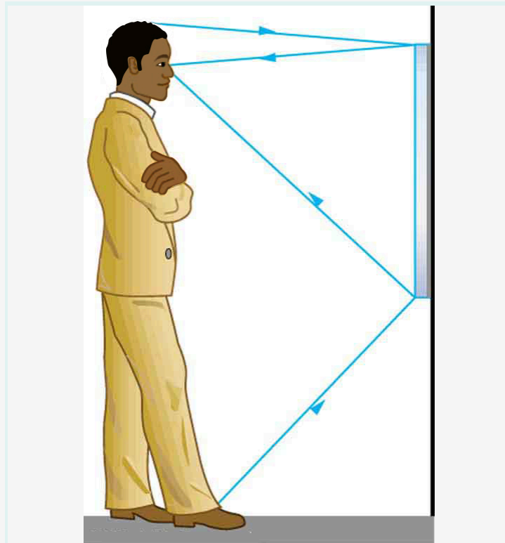
Figure 2: A full-length mirror is one in which you can see all of yourself. It need not be as big as you, and its size is independent of your distance from it.
