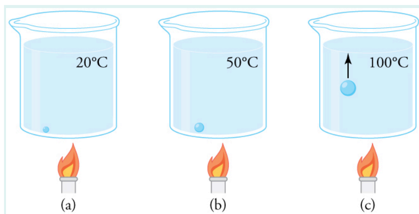
Figure 3: (a) An air bubble in water starts out saturated with water vapor at 20^\circ\text{C} . (b) As the temperature rises, water vapor enters the bubble because its vapor pressure increases. The bubble expands to keep its pressure at 1.00\text{ atm} . (c) At 100^\circ\text{C} , water vapor enters the bubble continuously because water's vapor pressure exceeds its partial pressure in the bubble, which must be less than 1.00\text{ atm} . The bubble grows and rises to the surface.
